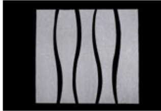
Figure 34: Cut gores to suit exact circumference of pipe. Remember to allow a half starter / finisher piece.
